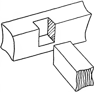
GAINED JOINT
